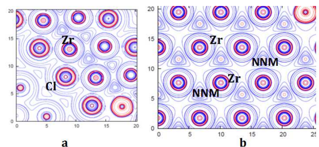
Figure 5. Laplacian, \nabla^2\rho_b plots of (a) Zr-Cl plane, (b) Zr-Zr plane.
